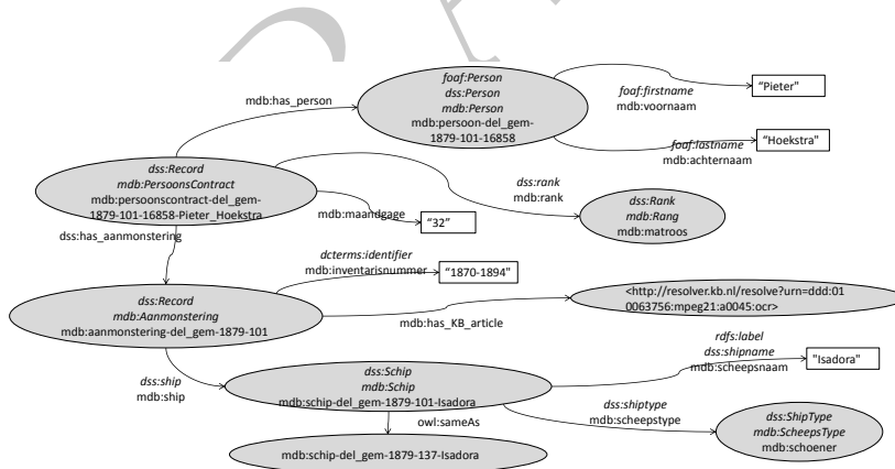
Fig. 3. Small sample of the RDF graph for MDB showing a person-contract and linked person; the counting (musterung) and a linked ship. Also shown are an internal owl:sameAs and an external link to a KB newspaper resource. For a number of properties, we list the DSS-superproperties in italics.
