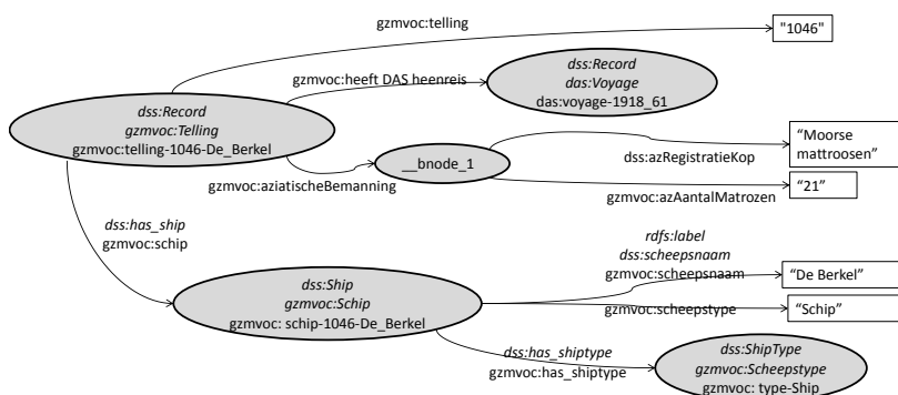
Fig. 2. Small sample of the RDF graph for GZMVOC showing a counting, a linked ship and detailed counting information connected to a blank node. Resources are represented using ovals, with the URI at the bottom line under italicized superclasses above, properties are represented by arrows, with property URIs next to them and their superproperties italicized. Literals are represented using boxes.
